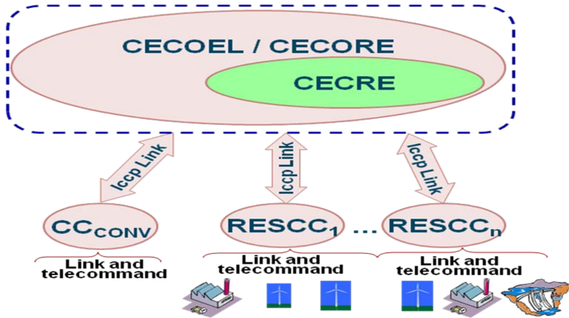
Figure 88. Functional Scheme of CECRE and RESCCs (Source: REE)
