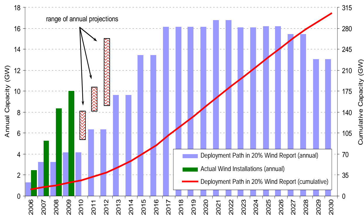
Figure 11. Potential U.S. Trajectory to Achieving 20% of Electricity from Wind Power by 2030 (Source: Provided by Ryan Wisler, Lawrence Berkley National Laboratory)
