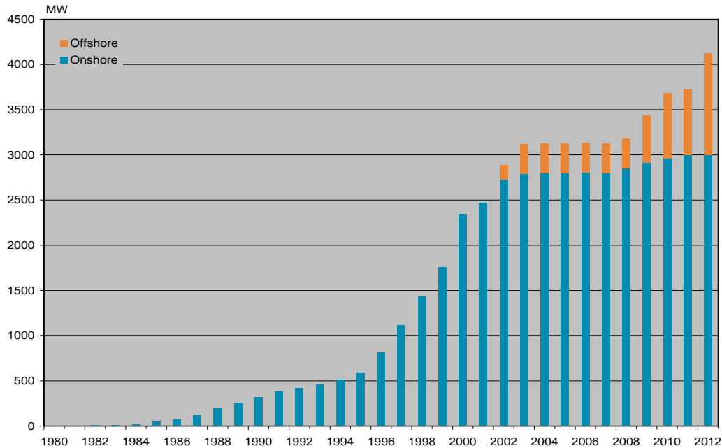
Figure 69. Cumulative Installed and Projected Wind Capacity in Denmark (Provided by Thomas Krogh, Energinet)
